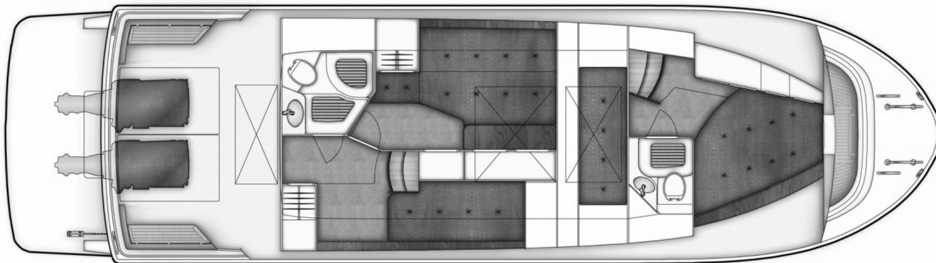
LOWER DECK
